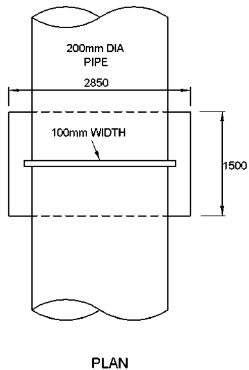
Figure13 Antifloatation block
