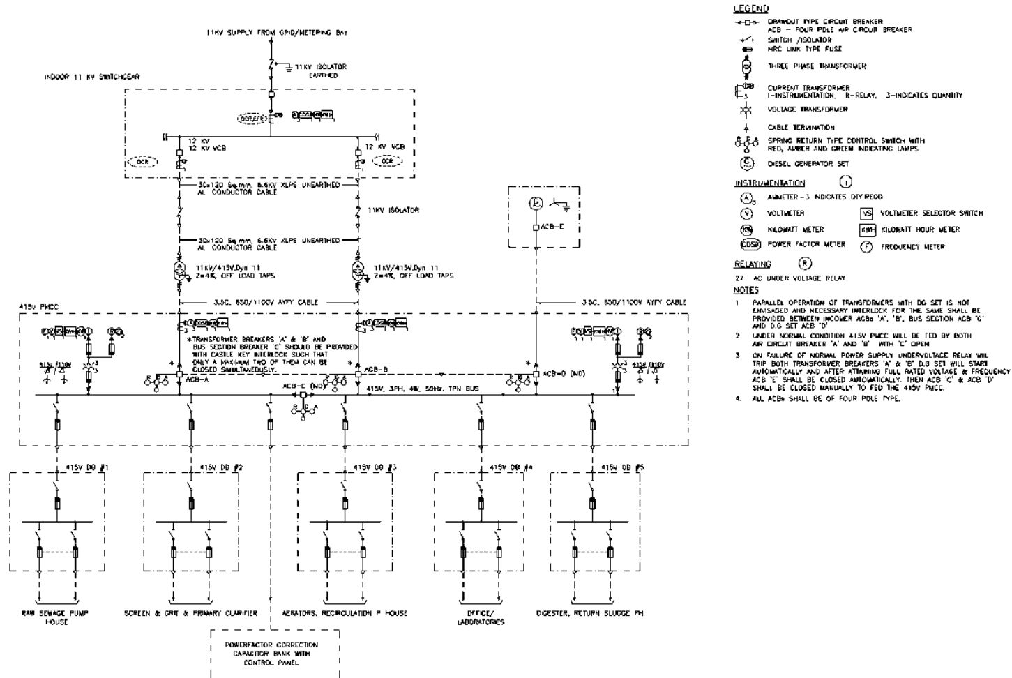
Figure 5.46 Typical electrical single line diagram for 11 KV/415 V transformer station with indoor KIOSK on 11 KV side showing relay connections to DG panel, symbol descriptions and notes
