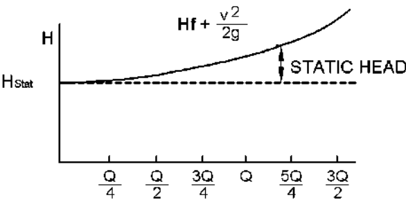
5625 Figure 4.6 System head curve for a pumping system
