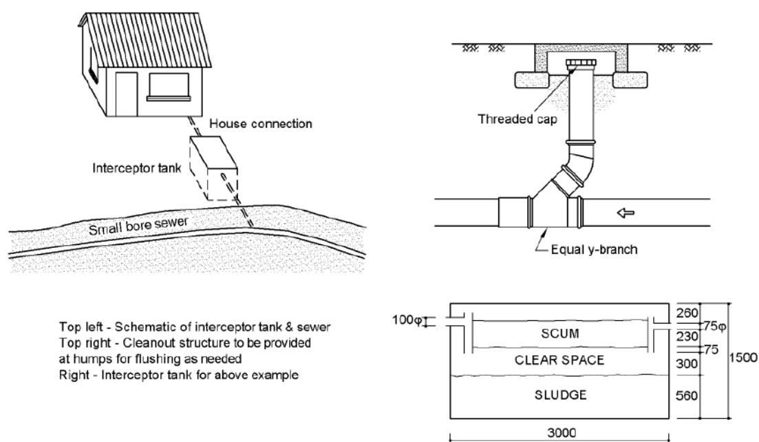
Figure 8.7 Schematics of small bore sewer system
