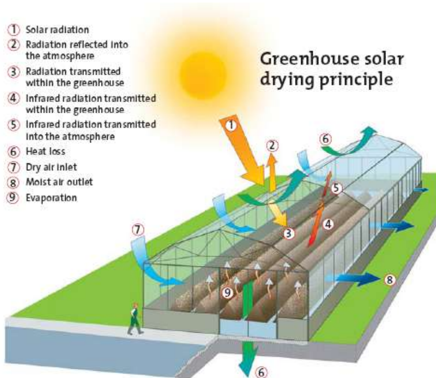
Figure 6.23 Typical operations in solar sludge drying
