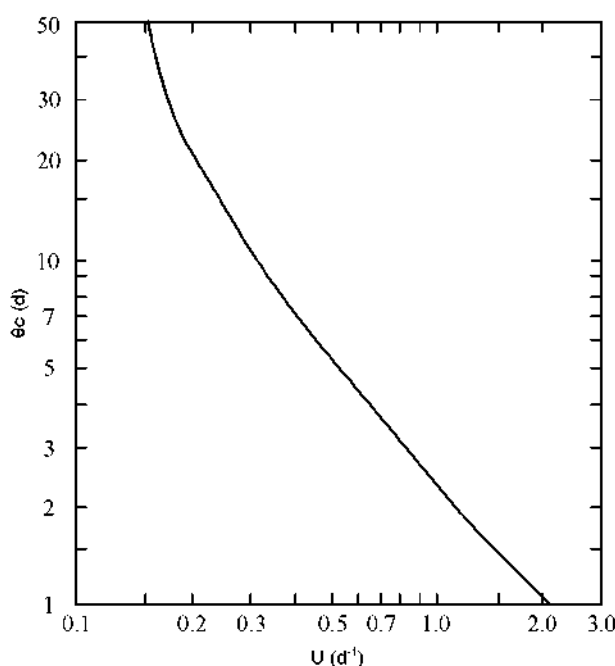
Figure 5.30 Relationship between SRT ( \Theta_c ) and specific substrate utilization rate ( U ) for Y = 0.5 and k = 0.06d^{-1}
