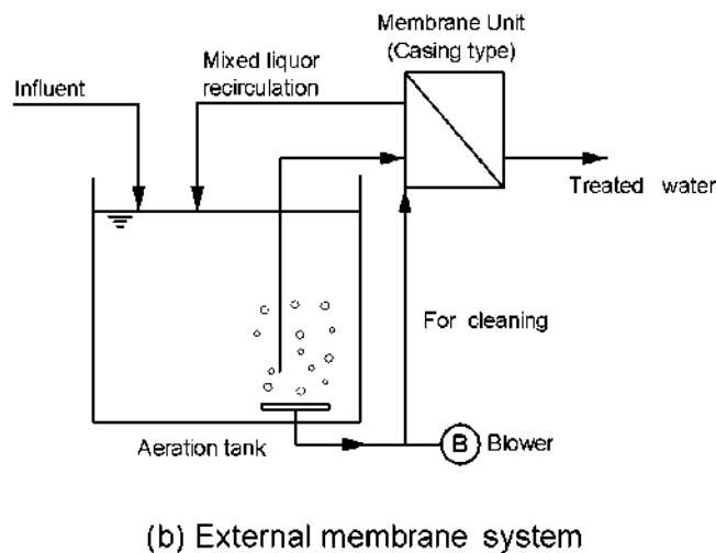
10860 Figure 5.67 Configuration of membrane bioreactor system
