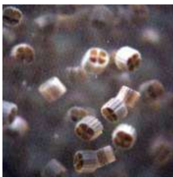
Figure 5.77 Kaldnes biofilm carriers (About 10 mm diameter \times 7 mm height)
