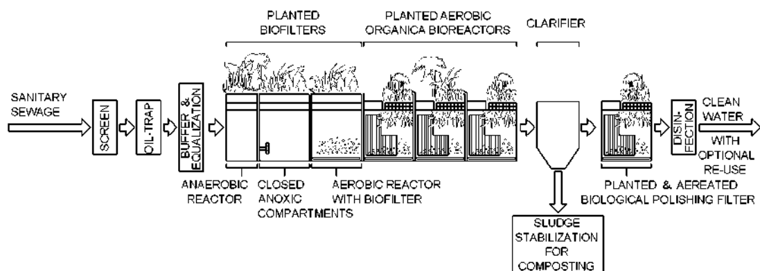
Figure 5.82 Organica cascade process
