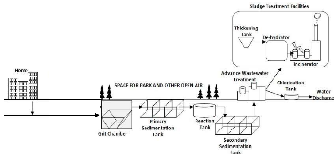
14845 Figure 7.14 Sequence of treatment units in Ochiai Water Reclamation Facility for wastewater reclamation
