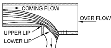
Figure 3.16 Leaping weir
