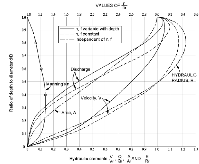
2600 Figure 3.12 Hydraulic – Element graph for circular sewers
