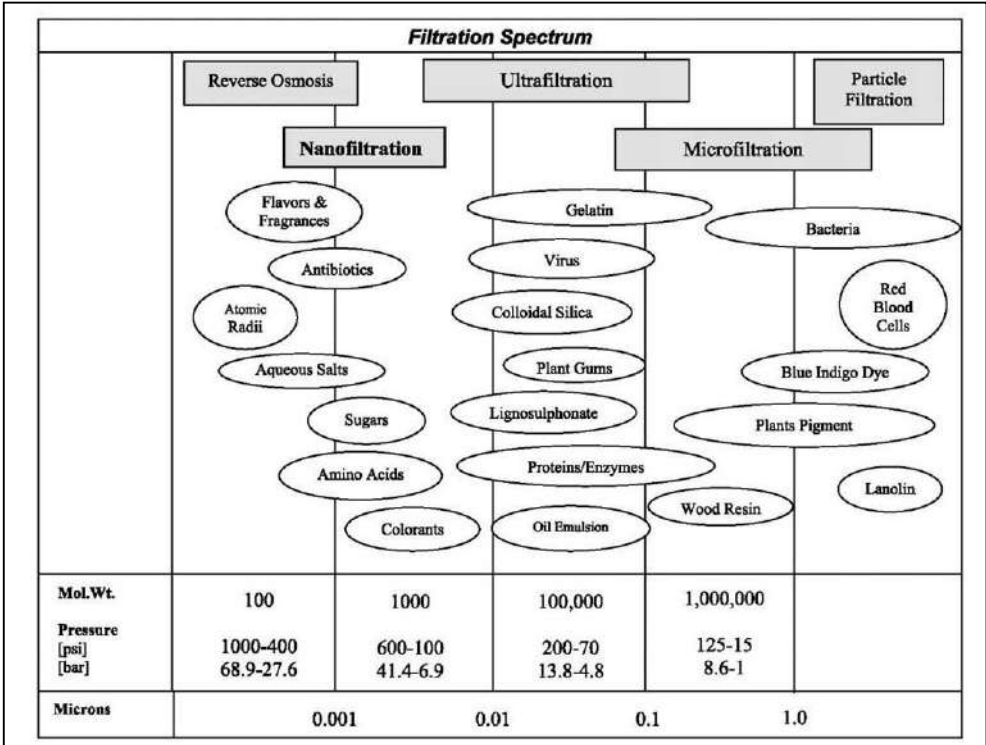
1855 Membrane filtration spectrum
