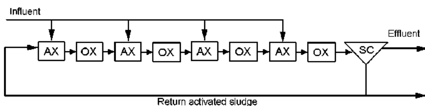
Figure 5.61 Step feed schematic for four pass anoxic-oxic system in Stamford
