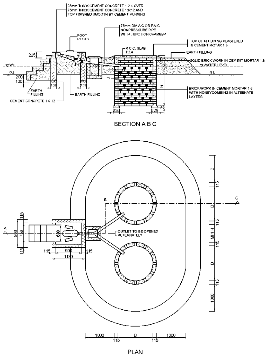
Figure 9.5 Pour flush latrine in water logged areas
