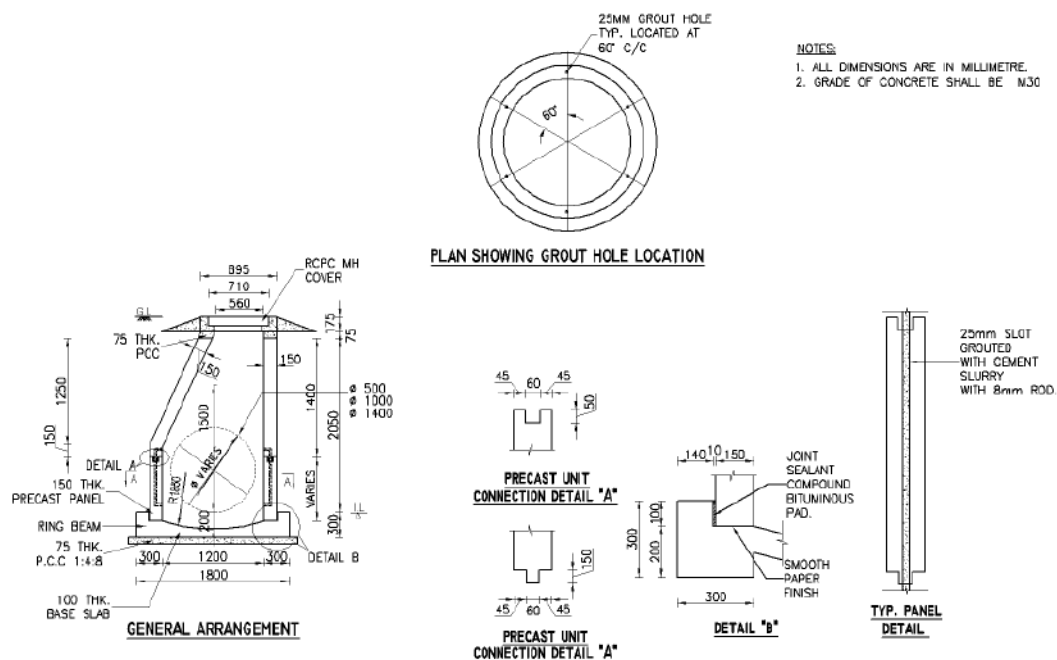
Figure 3.27 RCC Manhole for a depth between 0.6 m to 2.3 m
