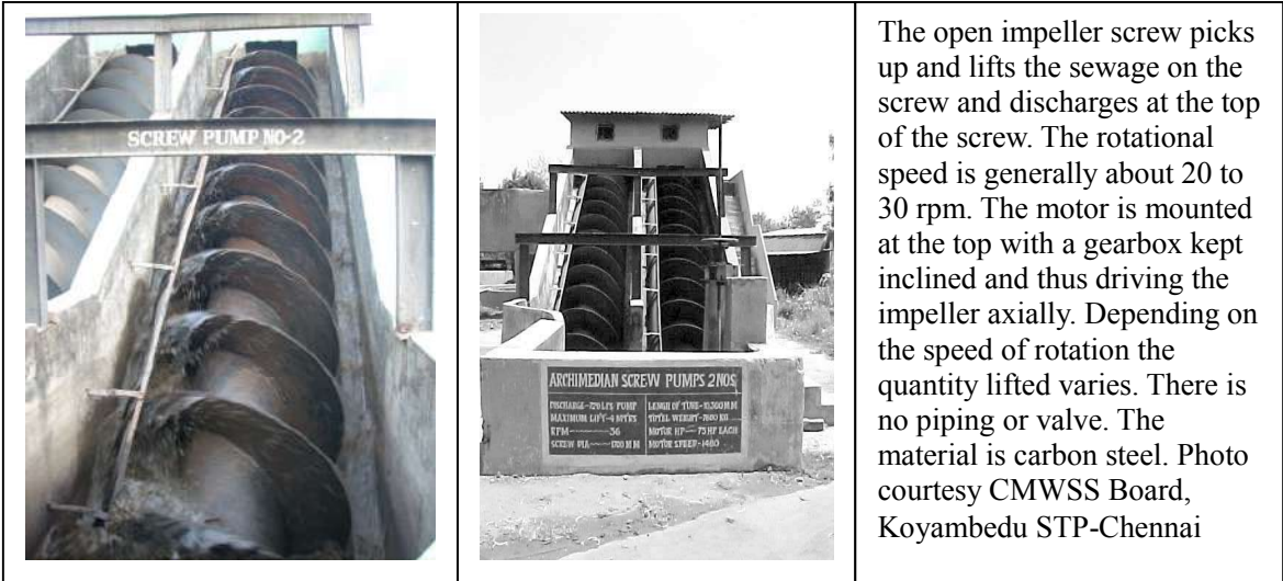
Figure 4.4 Archimedian screw pump.
